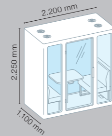
Duo Pod (with standing table and bench)
