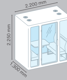
Meeting S (with standing table and bench)
