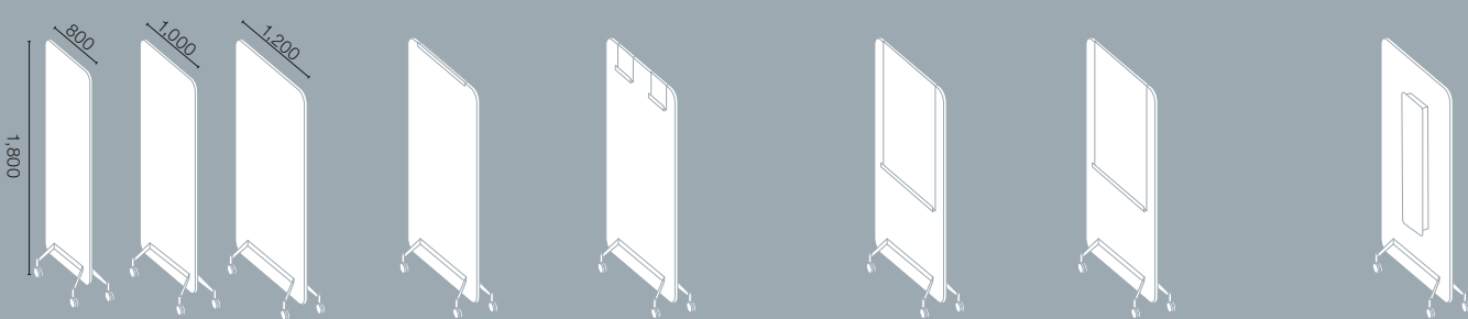
Mobile partition Mobile partitioning screen with track Mobile partitioning screen with 2 flipchart holders Mobile partitioning screen whiteboard Mobile partitioning screen metal panel, can be used as adhesive surface for magnets Mobile partitioning screen set up for TV
