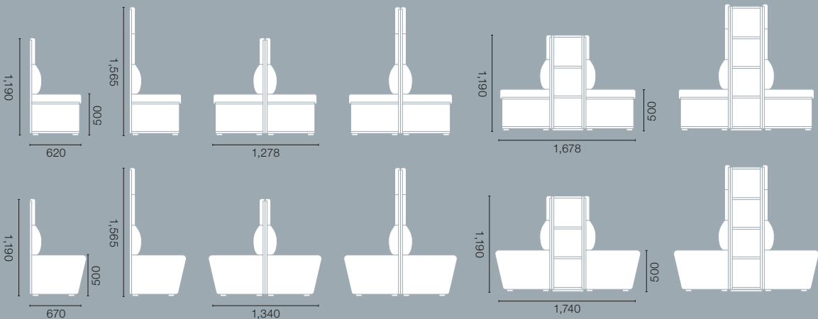
Diner Width: 800 / 1000 / 1,200 mm
