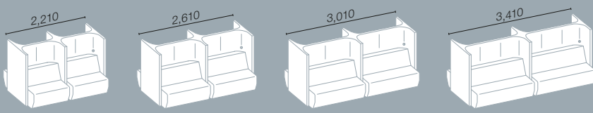
Quad lounge element Height 1,400 mm | Depth 1,570 mm
