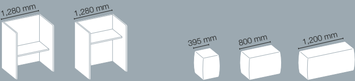
Temporary work stations Height 1,560 mm | Depth 800 mm
