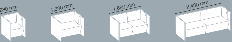
Seating lounge Height 930 mm | Depth 800 mm
